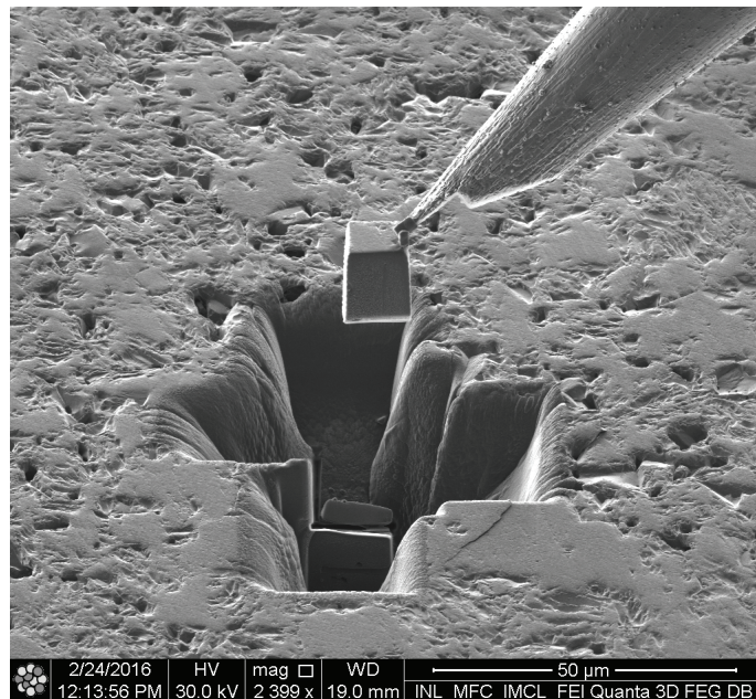
Figure 4. 10 micro-meter sample of irradiated uranium oxide fuel being lifted out in a focused ion beam for microstructural characterization.
